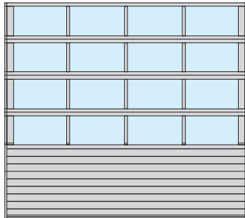
GATE WITH PANELS WITH ALUMINIUM GLAZED SECTION
