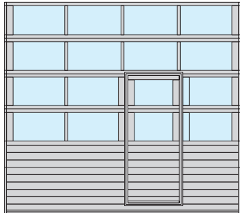
GATES WITH PASSAGE DOORS AND PANELS WITH ALUMINIUM GLAZED SECTION
