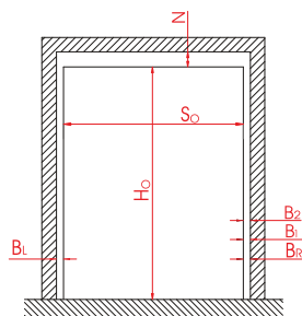
INTERNAL VIEW
