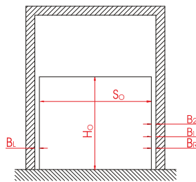
INTERNAL VIEW
